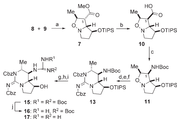
Scheme 3. Synthesis of bis-monocyclic guanidine 16 : a) toluene, 80°C (93%); b) LiOH, THF/H 2 O, 0°C; c) 1. (COCl) 2 , DMF (cat.), toluene; 2. NaN 3 , acetone/H 2 O, 0°C; 3. 1,4-dioxane, 100°C, then 10% HCl, then (Boc) 2 , K 2 CO 3 , (86% from 7 ); d) H 2 , Pd(OH) 2 , MeOH; e) NCBz=C(SMe)NHCbz ( 12 ), HgCl 2 , Et 3 N, DMF; f) DEAD, PPh 3 , toluene (97%, three steps); g) TFA, CH 2 Cl 2 ; h) NCBz=C(SMe)NHCbz ( 14 ), HgCl 2 , Et 3 N, DMF (77% two steps); i) TBAF, THF (92%); j) 5% TFA/CH 2 Cl 2 , 0°C ( 15 : 13%, 16 : 71%, 17 : 16%). Boc = tert -butyloxycarbonyl, DEAD = diethyl azodicarboxylate, Cbz = benzyloxycarbonyl, TBAF = tetrabutylammonium fluoride, TFA = trifluoroacetic acid.
